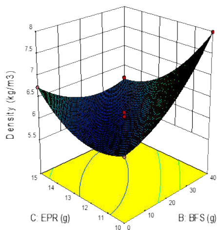
Fig. 7C: 3D plot of EPR and BFS for Density of sample
