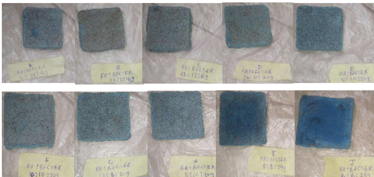
Fig. 3 Samples of fiberboard produced
