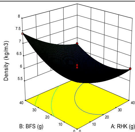
Fig. 7a: 3D plot of BFS and RHK for Density of sample
